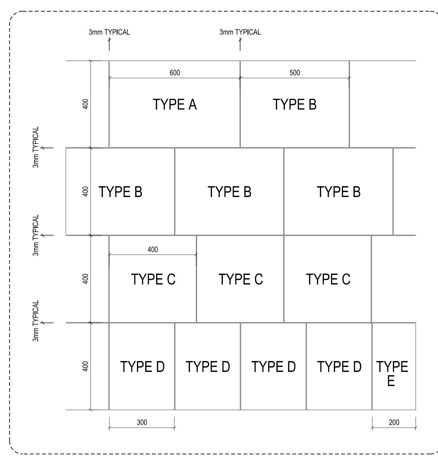
TL-06 TYPES SETOUT TYPICAL SCALE 1:10
